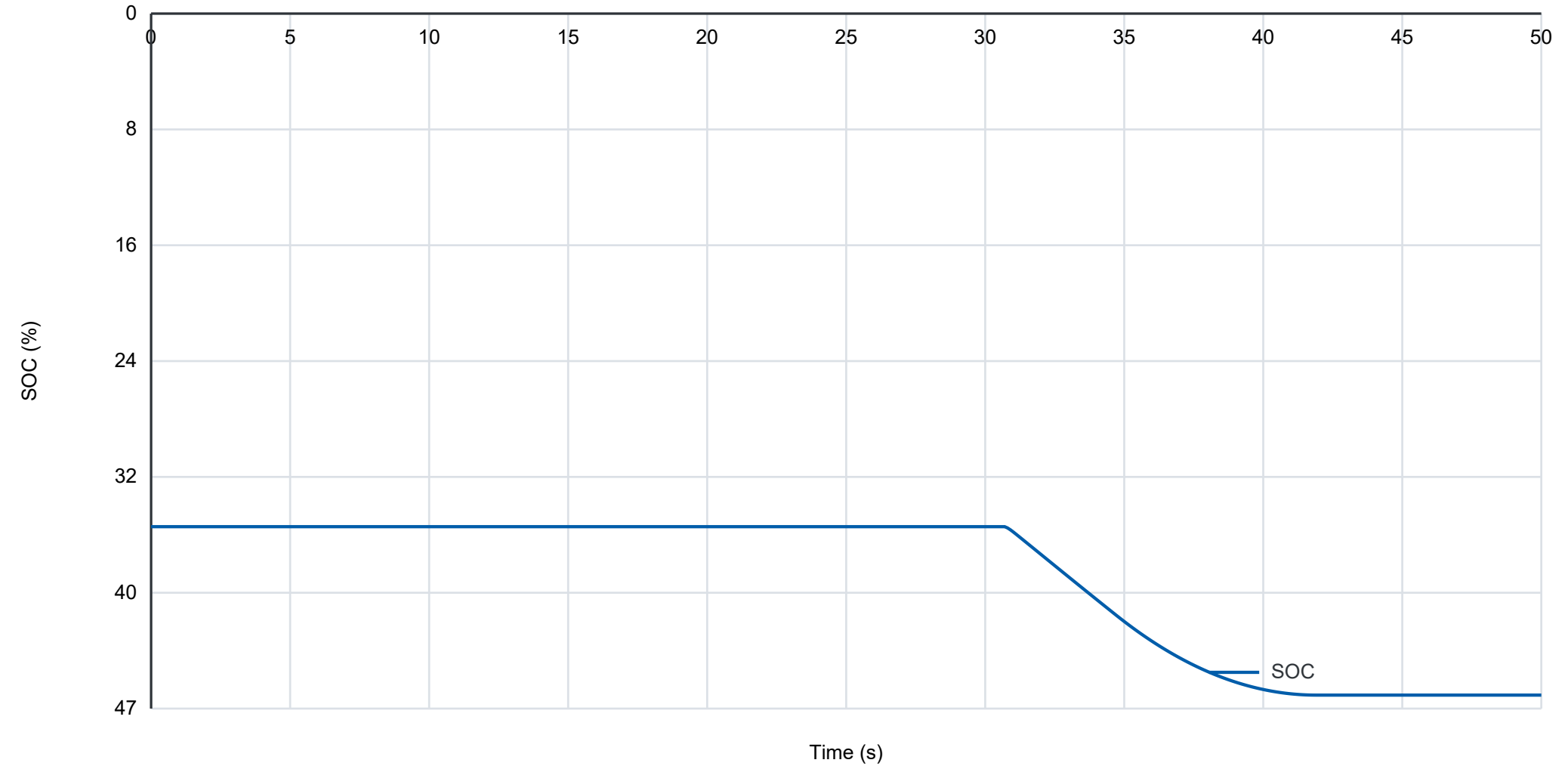
Supercapacitor SOC vs Time
