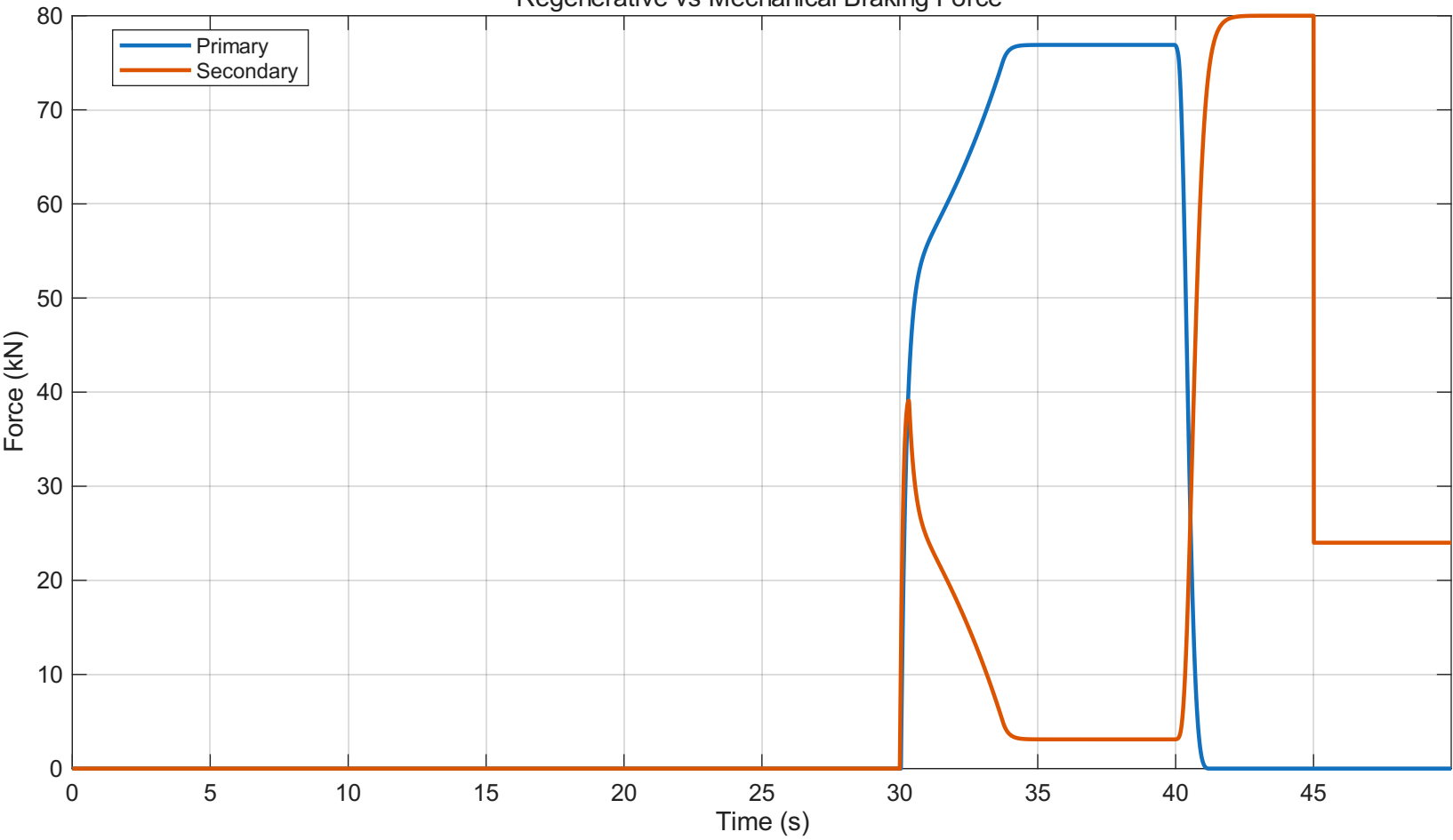
Regenerative vs Mechanical Braking Force
