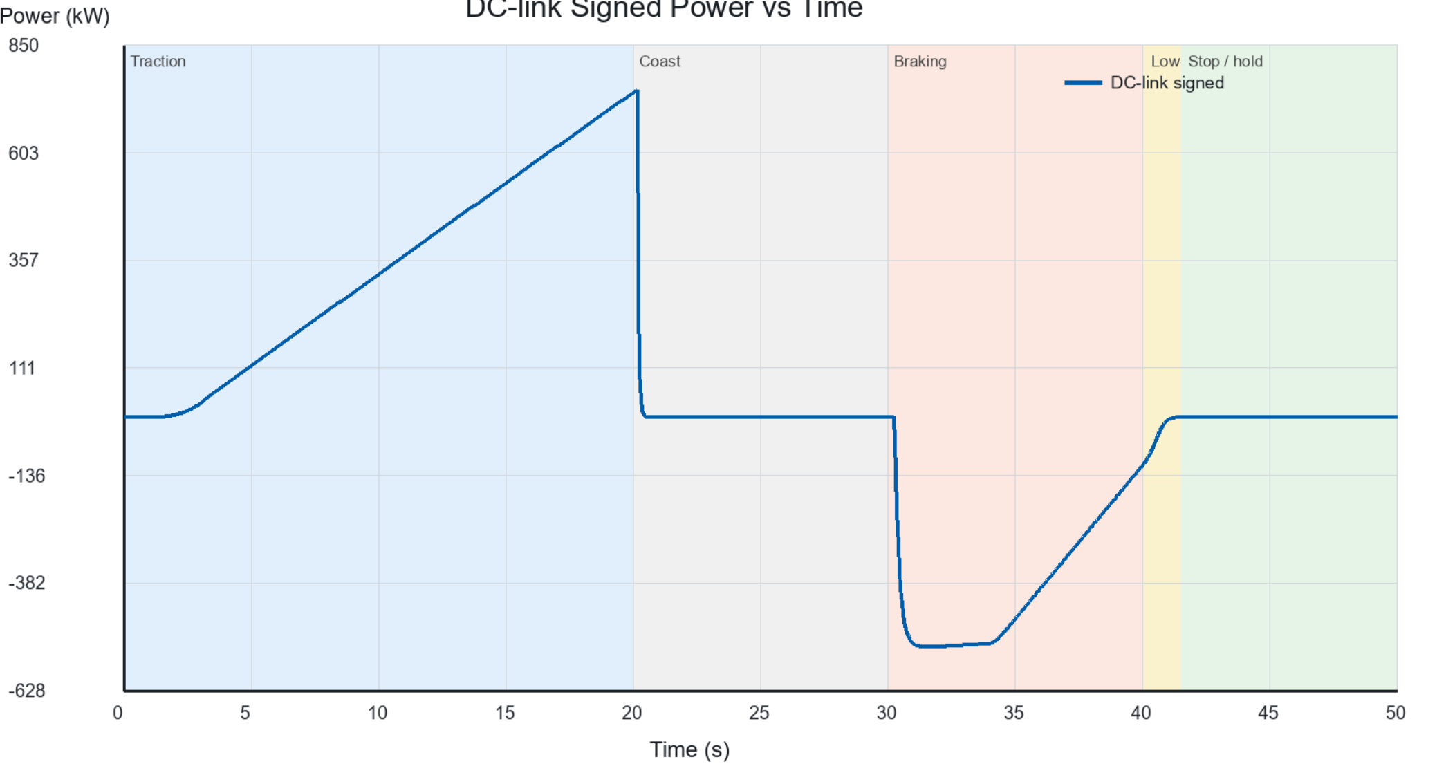
DC-link Signed Power vs Time
