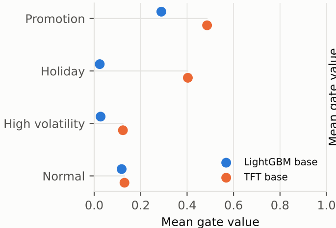
(a) Gate opens on promotions, closes under volatility
