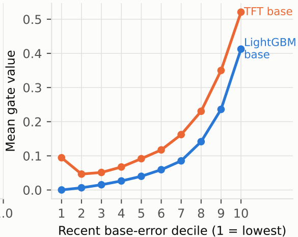
(b) Gate rises with recent base error
