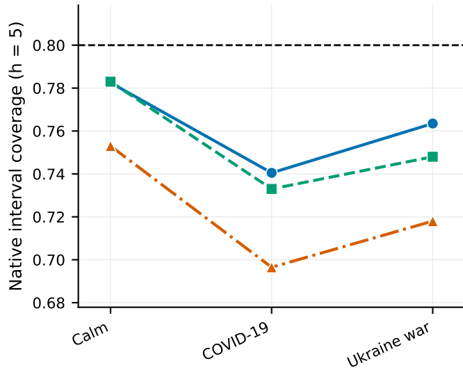
(b) Calibration degrades
