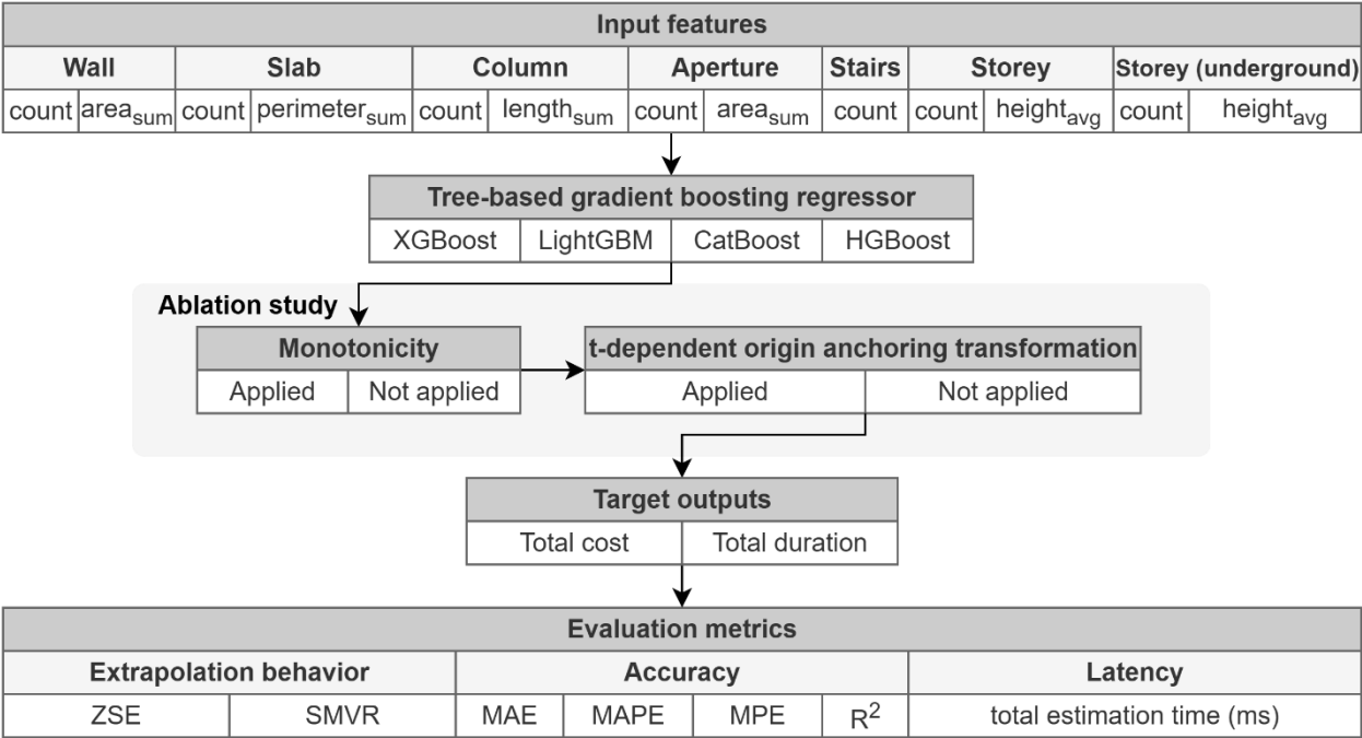
645 Fig. 9. Overview of ablation design, input features, target outputs, and evaluation metrics.
