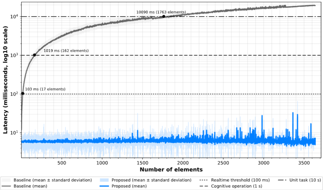
929 Fig. 11. Comparison of latency between state-log-based and BIM-model-based construction duration estimation 930 (CatBoost).
