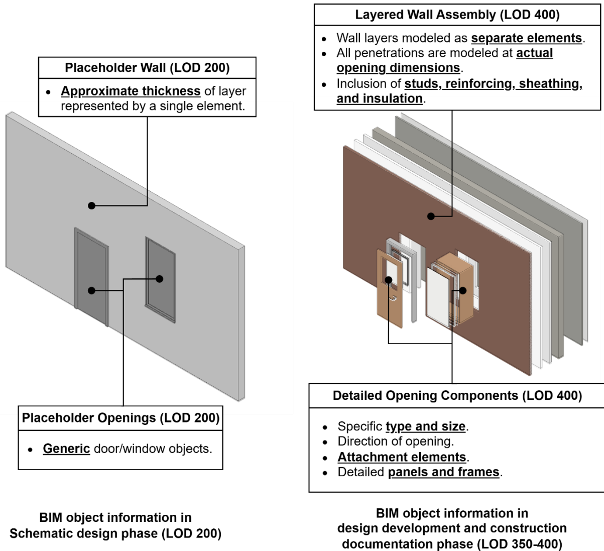
Fig. 1. Comparison of information granularity between LOD 200 (left), and LOD 400 (right) BIM elements (revised from Jang and Lee, 2024 [48]).
