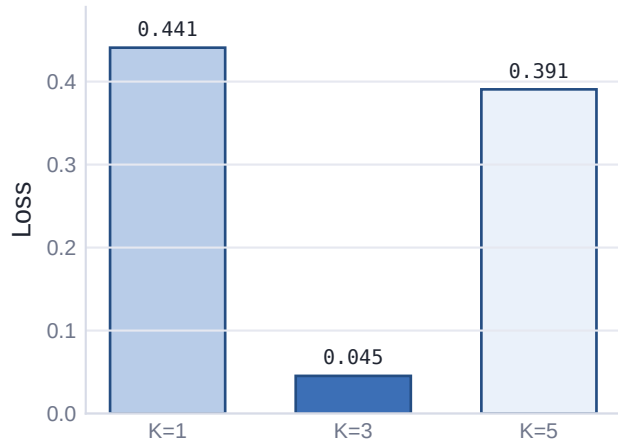
LFP loss
