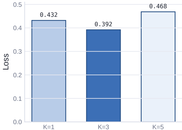
Action loss
