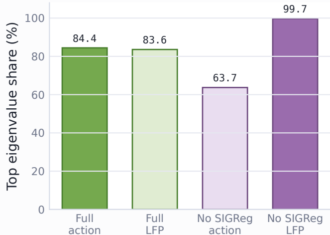
Variance concentration
