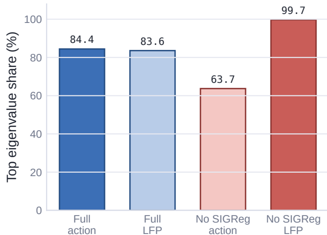
Variance concentration
