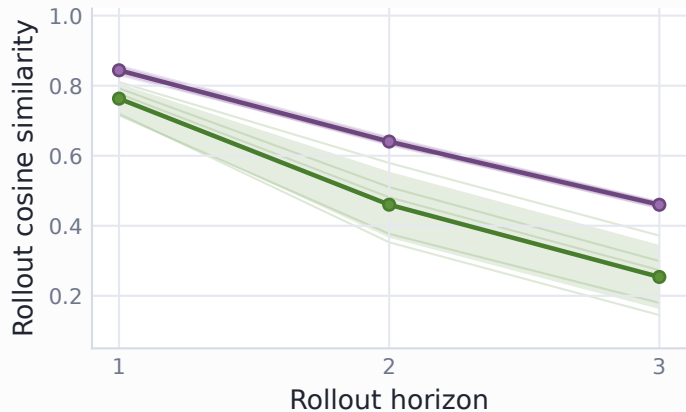
Action-selected checkpoint
