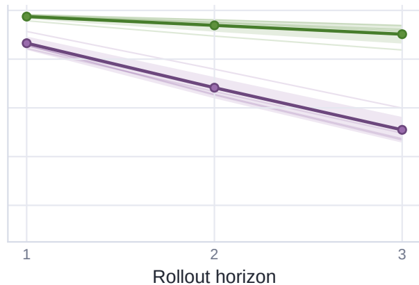
LFP-selected checkpoint
