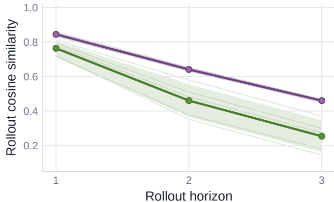
Action-selected checkpoint
