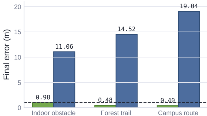
Goal-reaching accuracy
