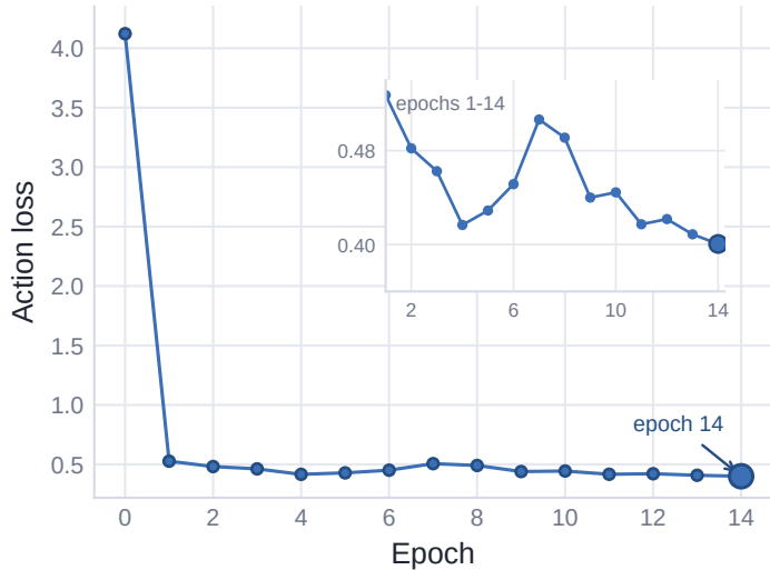
Action prediction
