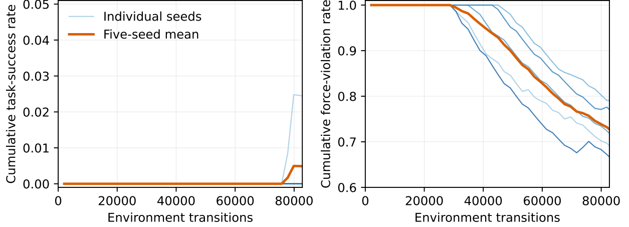
Fig. 2. Original matched-budget direct PPO training over five seeds and 82,774 environment transitions per seed.
