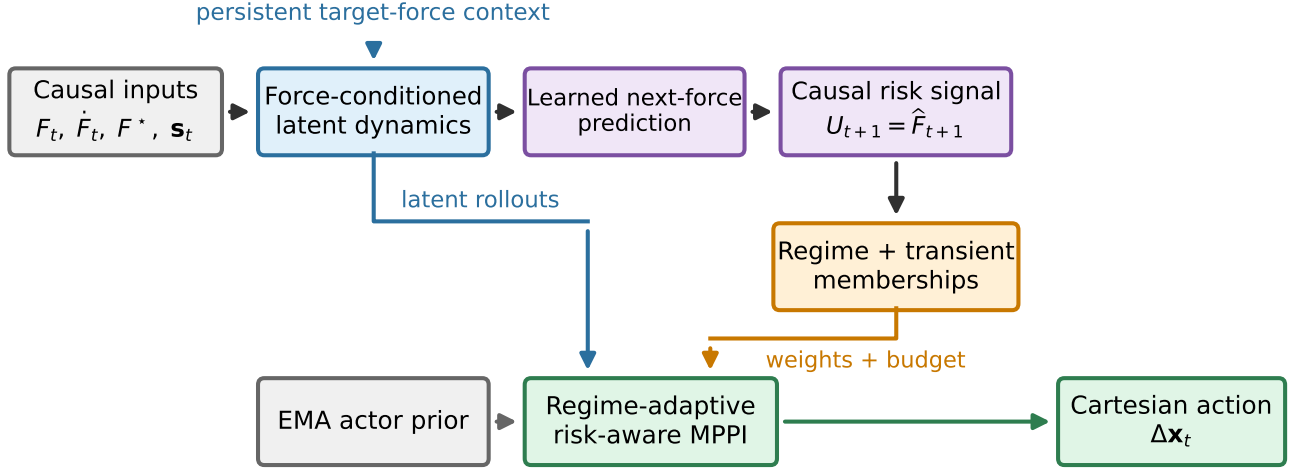
Fig. 1. Force-conditioned regime-adaptive risk-aware MPPI architecture.
