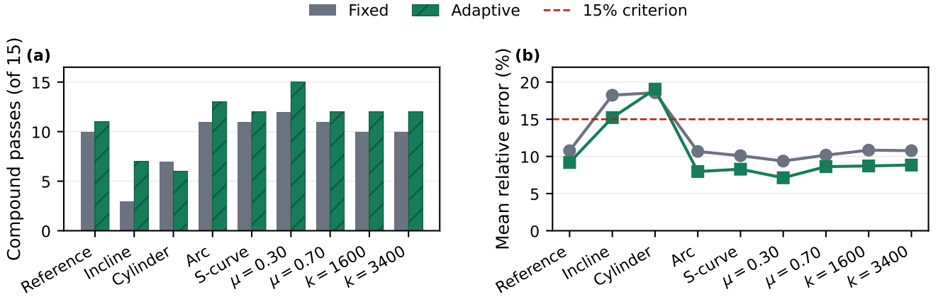
Fig. 3. Factor-separated task-and-tracking outcome and mean force error; 15 evaluations per factor level and planner.
