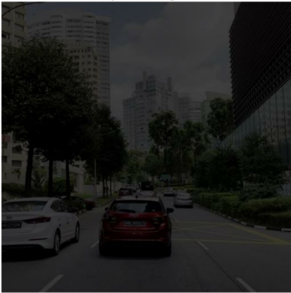
Input (Low-light)
