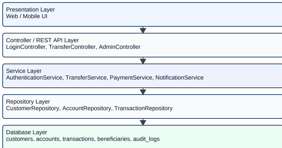
Figure 6: System Architecture Diagram
