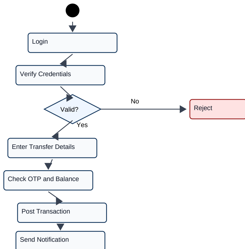
Figure 5: UML Activity Diagram
