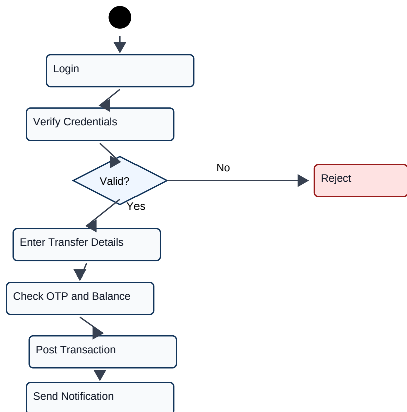
Appendix Figure A5: UML Activity Diagram
