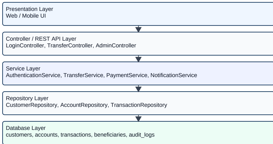
Appendix Figure A6: System Architecture Diagram
