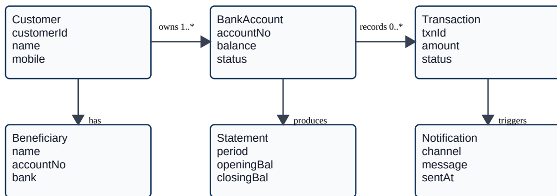
Domain Model Diagram
