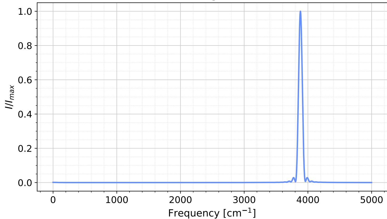
H 2 stretching QCT VDOS
