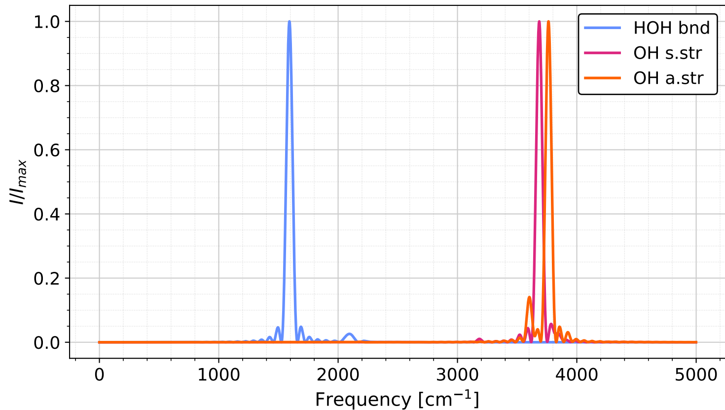
Normal mode VDOS of H 2 O
