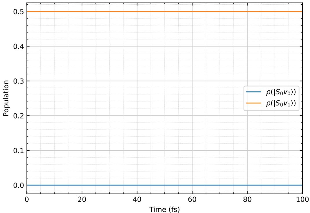
S_0 vibrational populations
