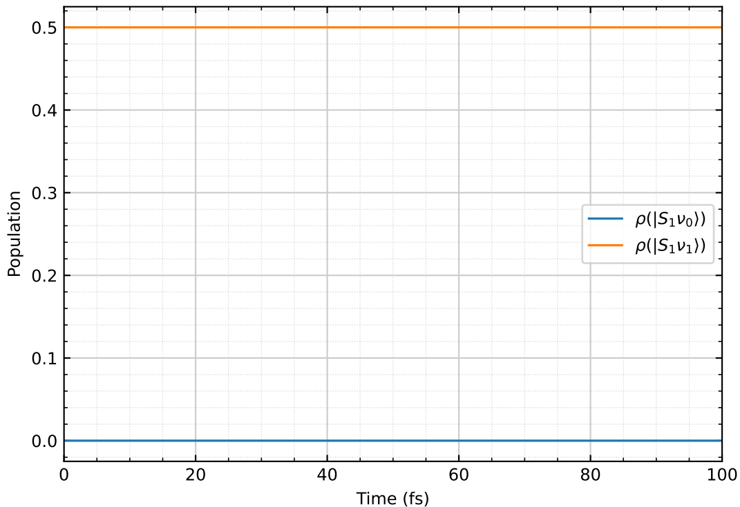
S_1 vibrational populations
