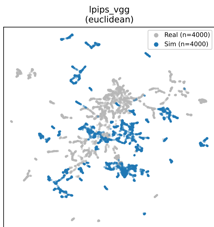
Cross-extractor overview (n_neighbors=20, min_dist=0.3)
