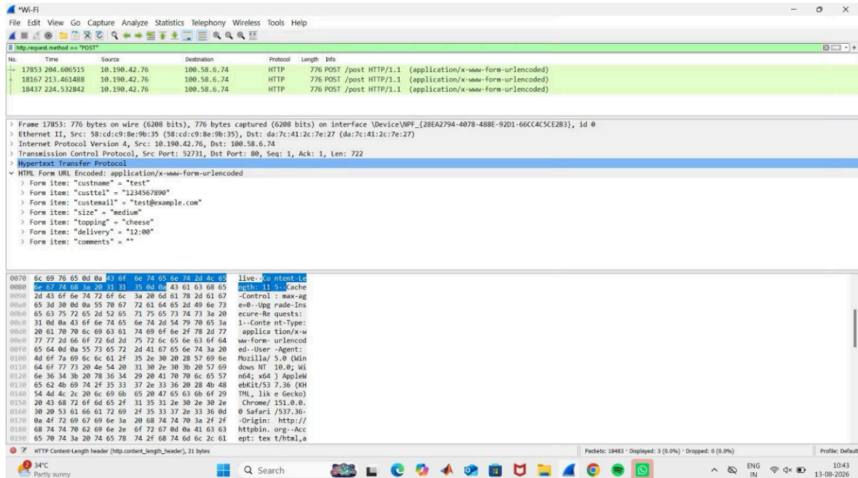
Figure 4: Plain-text Credential Extraction from Form Fields
