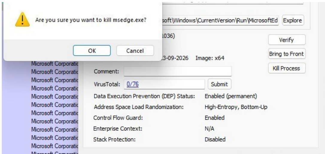
Figure5:Terminatingandsuspending maliciousprocesshandles
