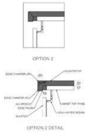
Gola Profile Option 2
