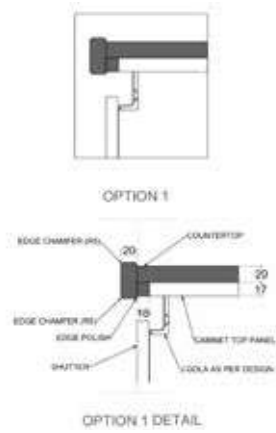
Gola Profile Option 1
