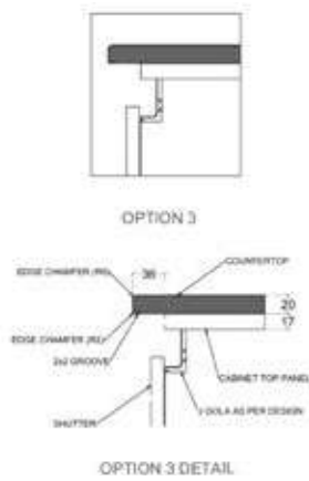
Gola Profile Option 3
