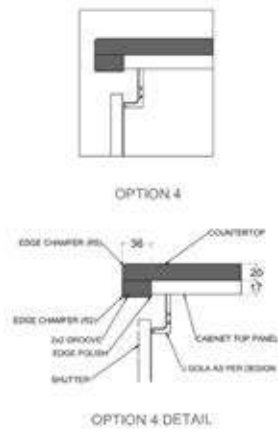
Gola Profile Option 4
