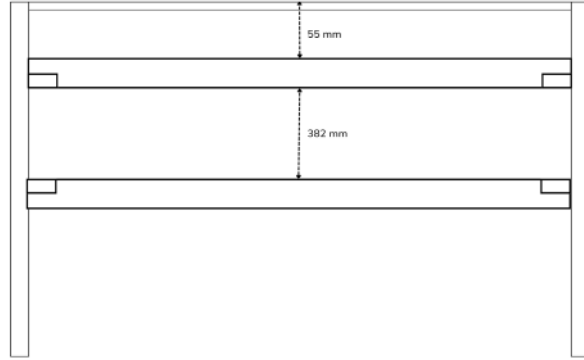
Position S4 (380 mm depth)
