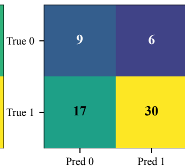
PATH — OS
