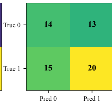
PATH — RT
