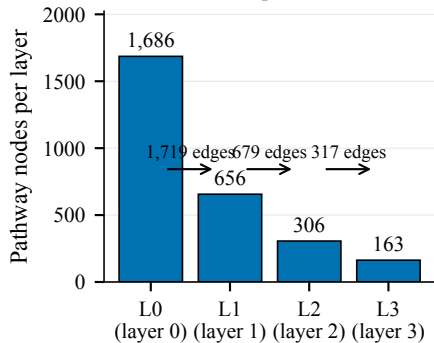
BINN — Reactome parent/child hierarchy
