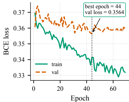
PATH (69 epochs)
