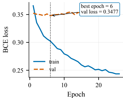
BINN (26 epochs)
