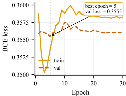
GraphPath (30 epochs)
