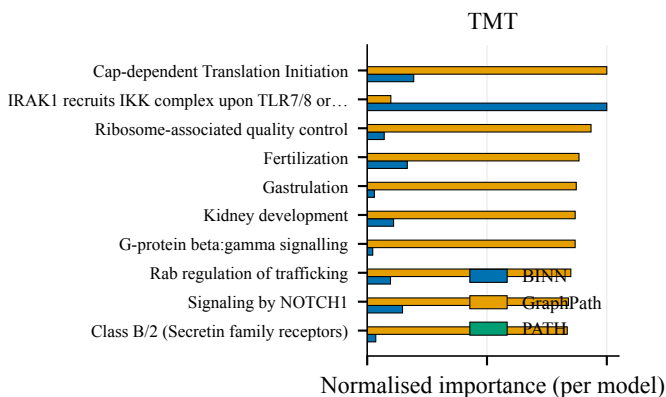
Top-10 pathways per head, ranked by union max importance across the three models (cohort: breast).
