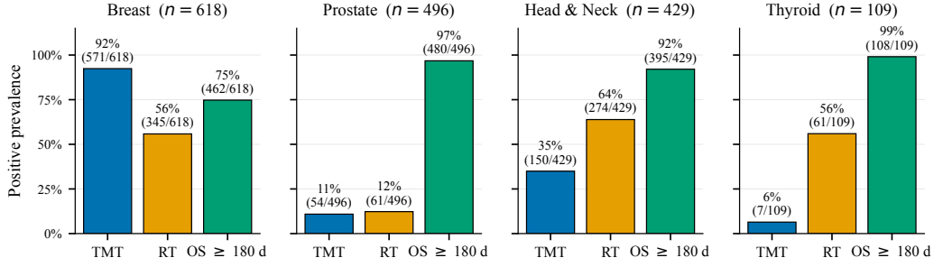
Fig. 1. Per-cohort positive prevalence of the three therapy-response heads, decoded from the stage bitfield of each cohort’s Final DataSet/CSV. Counts in parentheses are positives/total. Lung and bladder are present in the data but disabled in COHORT_FILES (see text); the four shown here are what the --cohort flag accepts.
