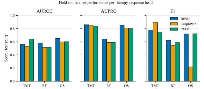
Fig. 3. Test-set AUROC, AUPRC, and F1 per therapy-response head. Bars in Okabe-Ito colours: BINN blue, GraphPath orange, PATH green.
