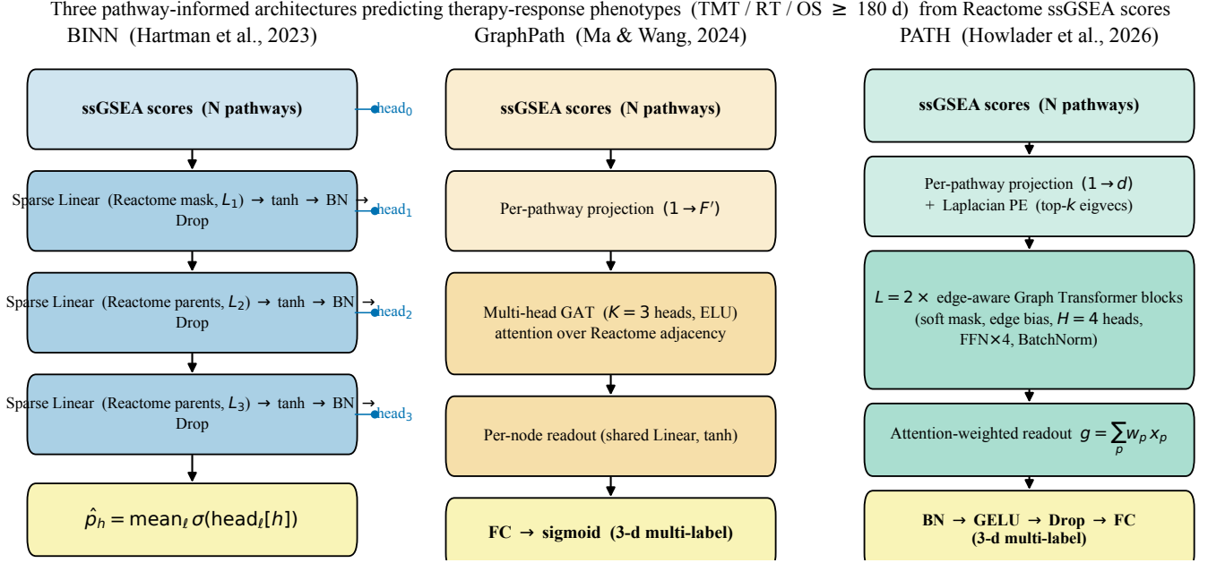
Fig. 2. Three pathway-informed architectures. BINN imposes the Reactome hierarchy via sparse masked-linear weights; GraphPath imposes pathway-pathway adjacency via multi-head GAT; PATH imposes the same adjacency through an edge-aware Graph Transformer with Laplacian positional encoding and edge-conditioned attention bias.
