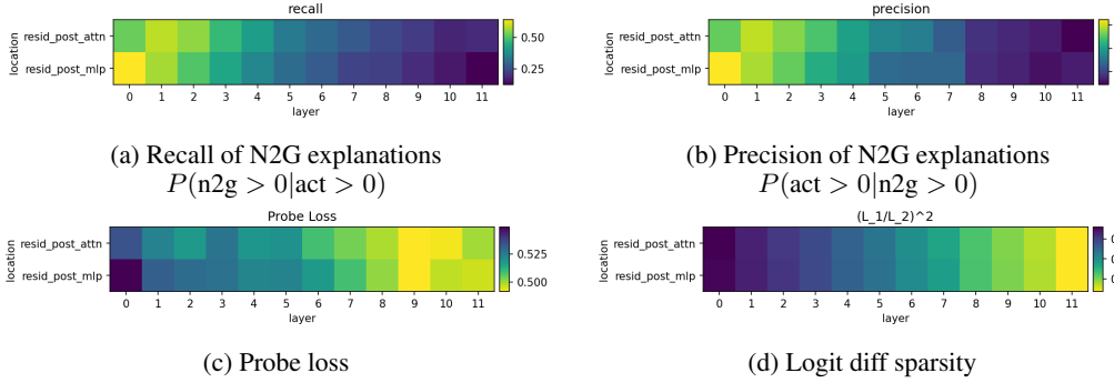
Figure 28: Metrics as a function of layer, for GPT-2 small autoencoders with k = 32 and n = 32768 . Earlier layers are easier to explain in terms of token patterns, but later layers are better for recovering features and have sparser logit diffs.
