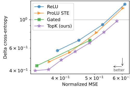
Figure 11: For a fixed sparsity level ( L_0 = 128 ), a given MSE leads to a lower downstream-loss for TopK than for other activations functions. (GPT-4). We are less confident about these runs than the corresponding ones for GPT-2, yet the results are consistent (see Figure 5).
