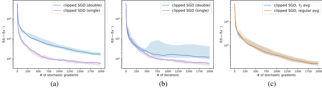
Figure 4: Ablations of Algorithm 1. Figures 4a and 4b compares single and double sampling by plotting sub-optimality as a function of gradient and iteration budget, respectively. Figure 4c compares different averaging methods. We plot the median across 10 runs, with a shaded region showing the inter-quartile range.
