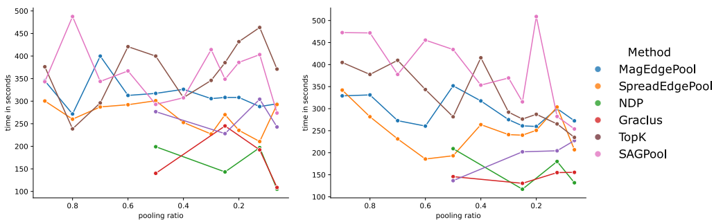
Figure S.3: Runtime comparison for training the GNNs reported in Section 4.1 for NC11 using different pooling layers. Plots show the mean time in seconds per run using general convolutional layers (left) or GIN layers (right).
