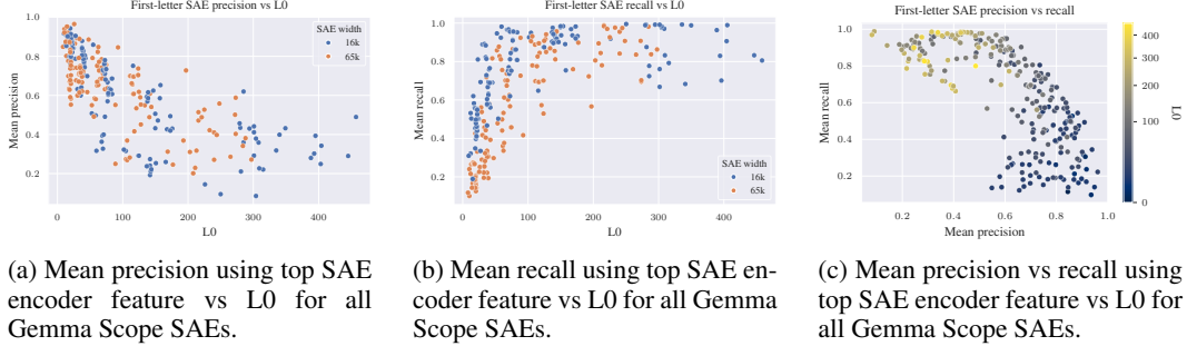
Figure 3: Precision and recall vs L0 for first-letter classification tasks
