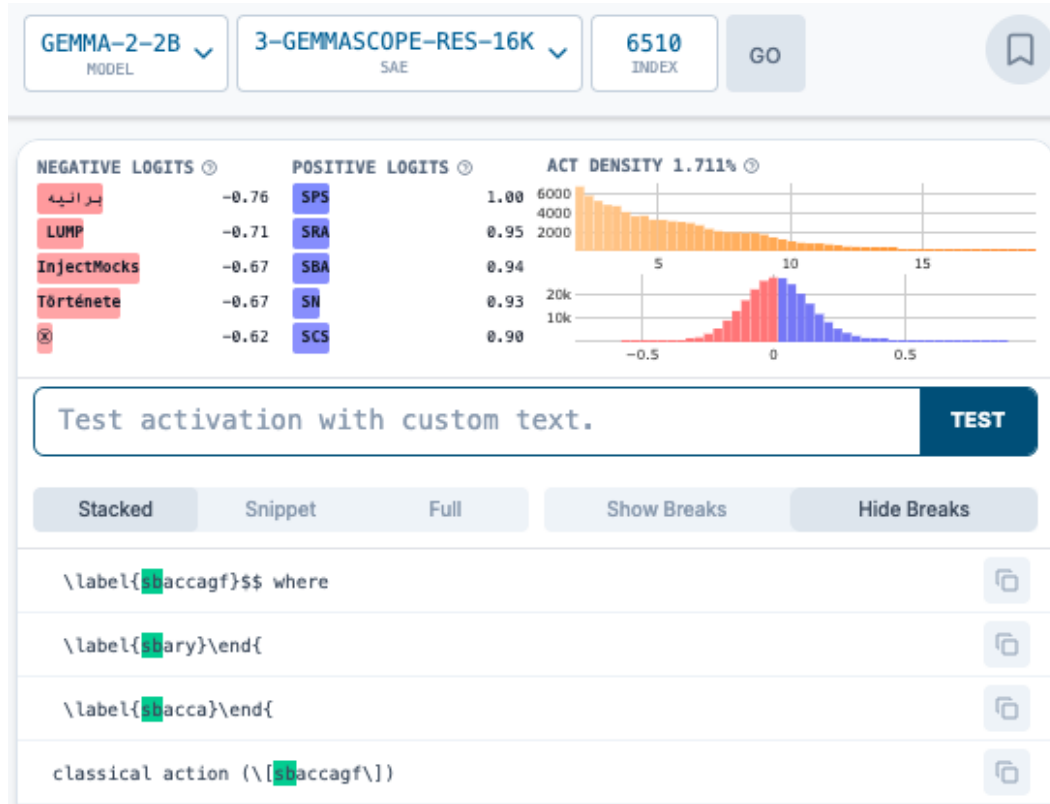
Figure 22: Neuronpedia dashboard for Gemma Scope layer 3, latent 6510. This latent should be the main “starts with S” latent.
