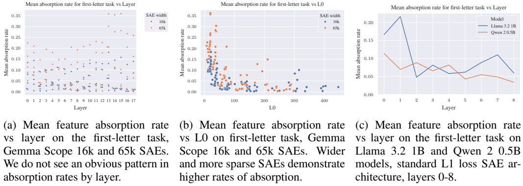
Figure 7: Feature absorption rates
