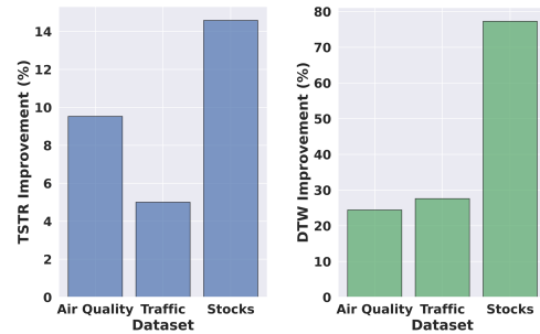
Figure 2: CPS outperforms existing approaches on real-world datasets. Dynamic Time Warping (DTW) measures the similarity between the real and the generated time series. The Train on Synthetic and Test on Real (TSTR) evaluates a task model on real test data when the model was trained on synthetic data. Improved TSTR indicates high generated sample quality. CPS provides 42% and 10% improvements for DTW and TSTR, respectively, over SOTA methods.
