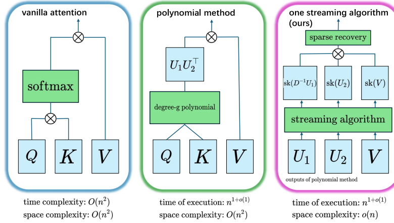
Figure 1: Comparison between our method and previous works. On the left: vanilla attention computation (Vaswani et al., 2017); Middle: fast attention by polynomial method (Alman & 2023a); On the right: one pass algorithm (ours).
