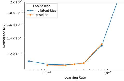
Figure 15: b_{\text{enc}} does not strongly affect loss (gpt2sm 128k, k=32 ).
