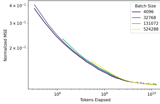
Figure 10: With correct hyperparameter settings, different batch sizes converge to the same L(N) loss (gpt2small).
