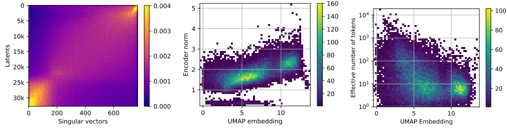
Figure 20: The residual stream seems composed of two separate sub-spaces. About 25% of latents mostly project on a sub-space using 25% of dimensions. These latents tend to have larger encoder norm, and to activate on a smaller number of vocabulary tokens. The remaining 75% of latents mostly project on the remaining 75% of dimensions, and can activate on a larger number of vocabulary tokens.
