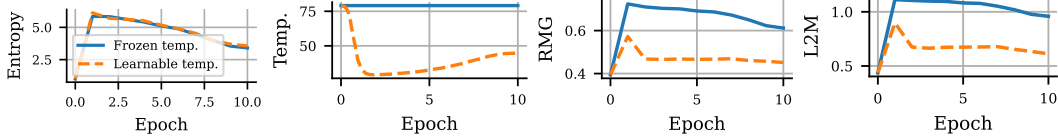
Figure 8: A model trained with frozen temperature increases the modality gap more than a model with trainable temperature to achieve a similar logit entropy.
