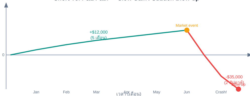
Short Vol P&L Path — Slow Gain / Sudden Blow-up
