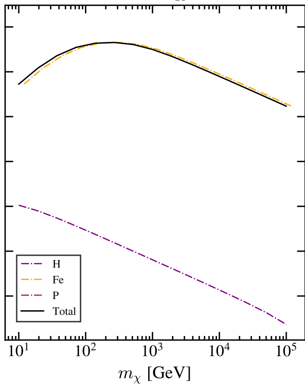
AGSS09: c_{15}^1 \neq 0
