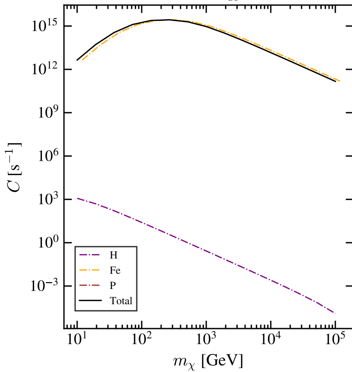
AGSS09: c_{15}^0 \neq 0
