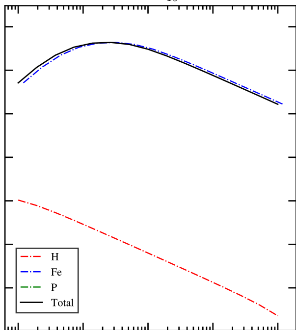
AGSS09: c_{15}^1 \neq 0
