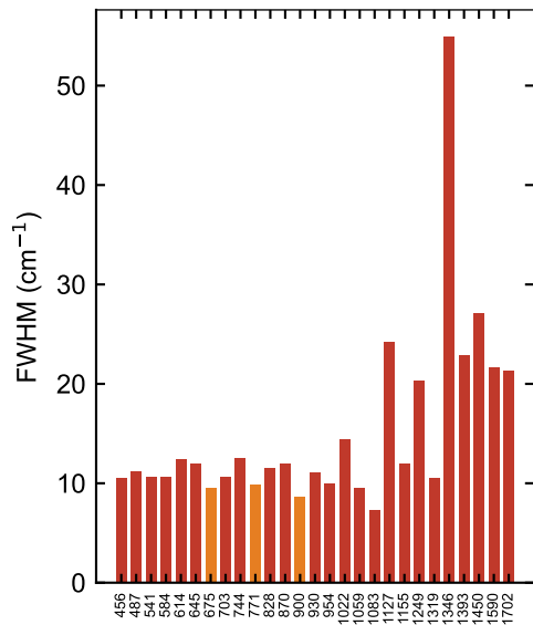
(c) Peak width (FWHM) from mean spectrum
