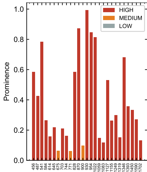
(a) Peak prominence Data: 70p-60s-5ac-diifrentpoint | n=3 spots
