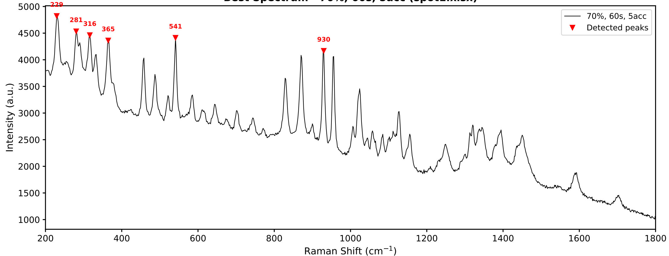
Best Spectrum - 70%, 60s, 5acc (spot1.xlsx)
