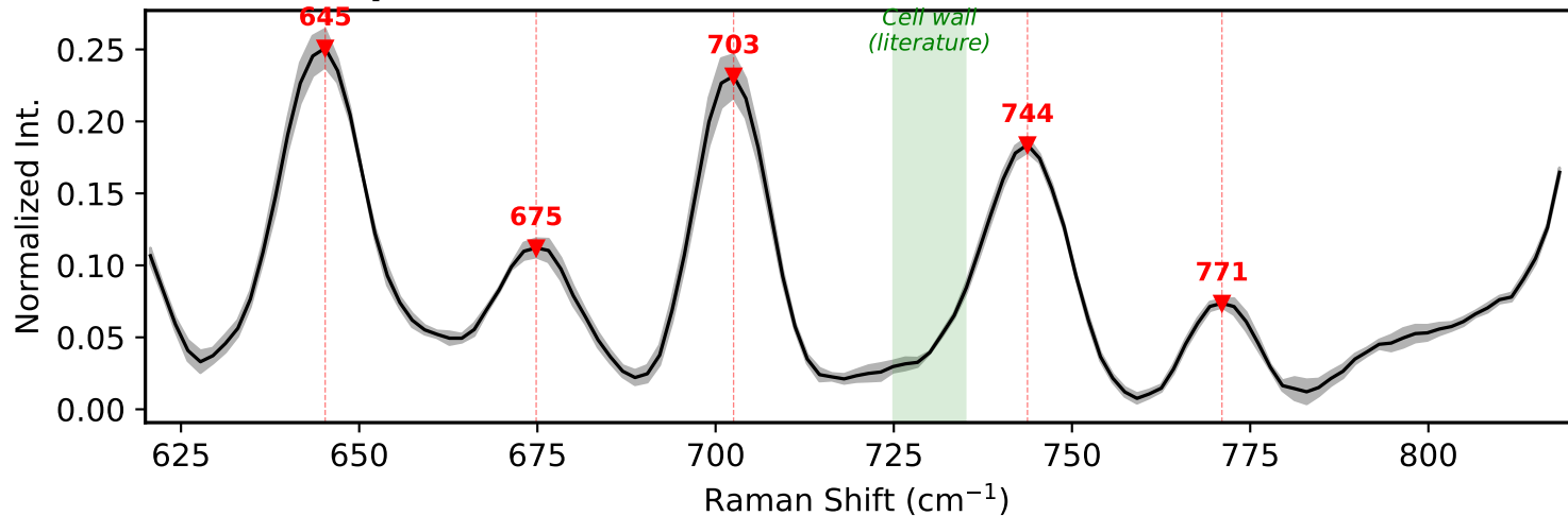
(c) Mean Spectrum with Peak Positions
