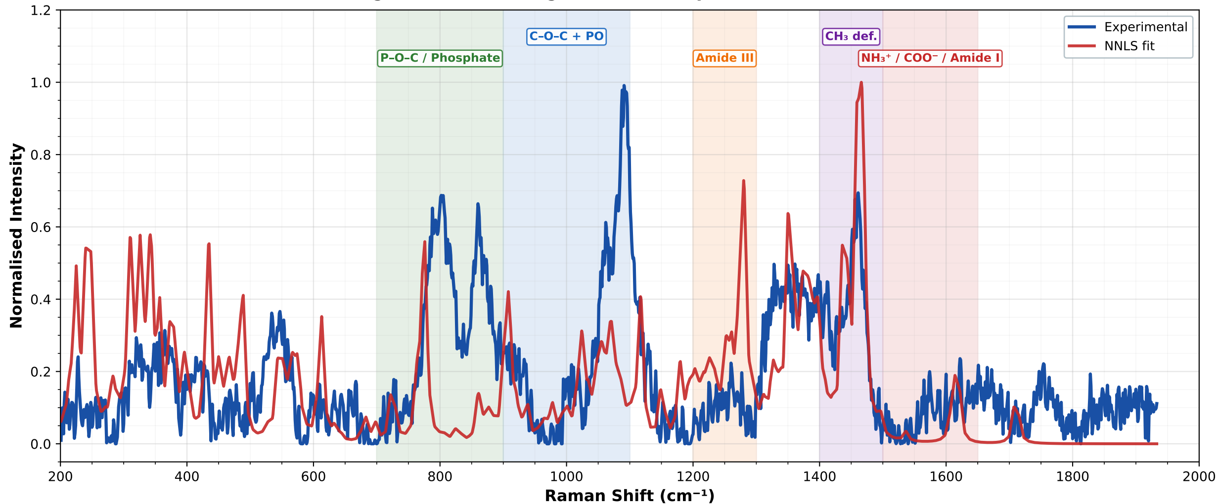
Diagnostic Raman Regions in LTA: Experimental vs NNLS Fit
