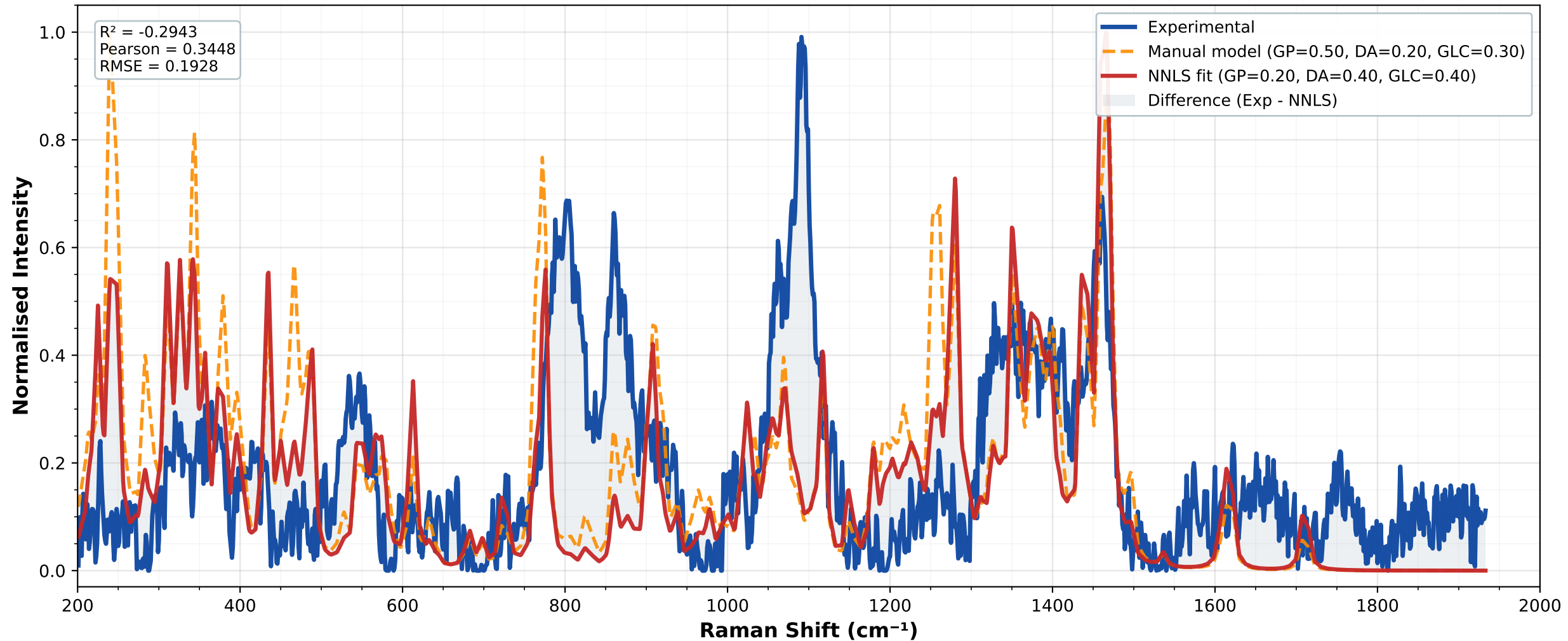
LTA Raman Spectrum: Experimental vs Manual and NNLS Models
