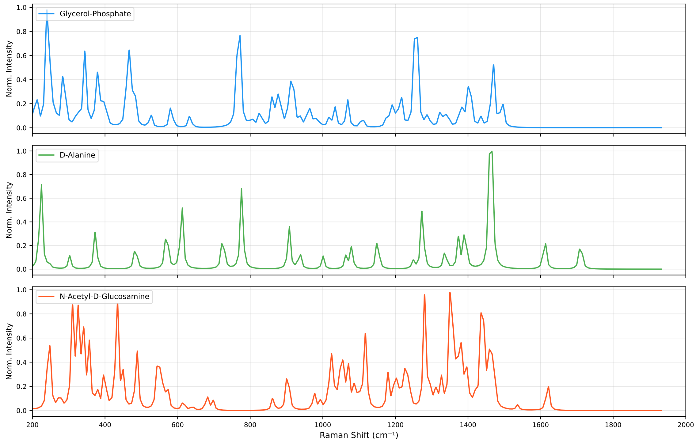
LTA Component Spectra (DFT-simulated, scaled & normalised)
