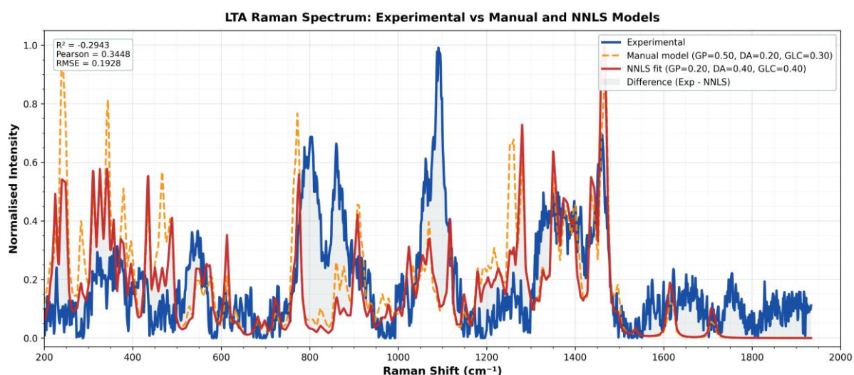
Figure 4. LTA experimental spectrum compared with manual and NNLS fragment models. The plotted fit metrics illustrate why the global model requires further refinement. Source: 20-04/lta/results/final_overlay.png.
