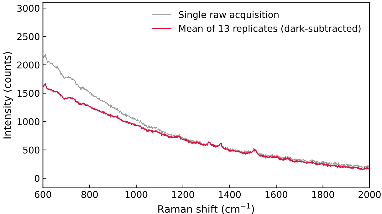
Figure 1. Raw CCD spectrum -- condition 5m-5ml-hf-5s-10p-5ac
