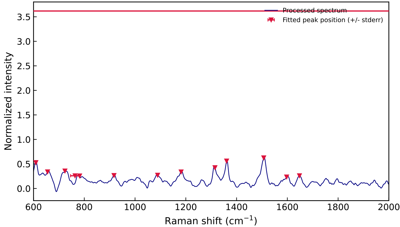
Figure 6. Fully processed experimental spectrum with fitted peaks (5m-5ml-hf-5s-10p-5ac)
